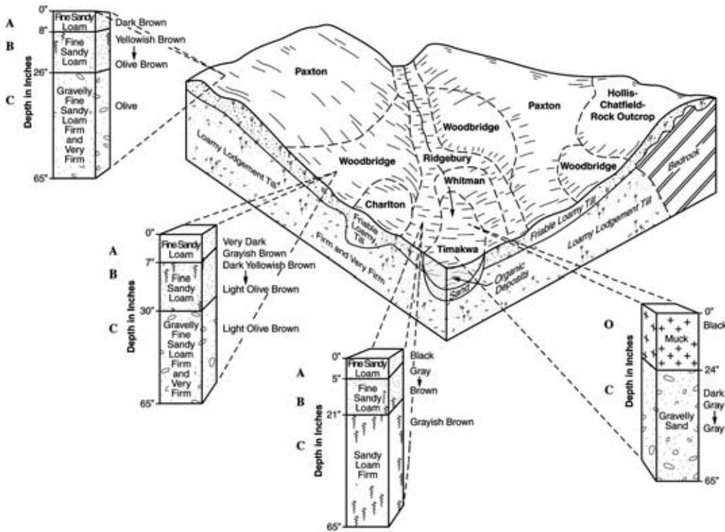
Figure 5.—Relationship of soils, landscapes, and parent material in the Paxton-Woodbridge-Hollis general soil map unit.
