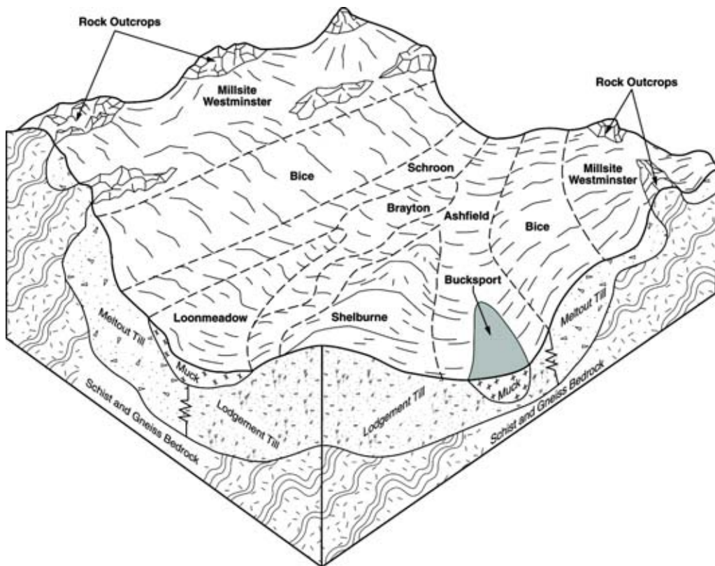
Figure 6.—Typical pattern of soils in the Bice-Millsite-Westminster general soil map unit and the Ashfield-Shelburne-Loonmeadow general soil map unit.
