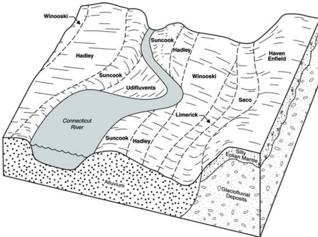
Figure 3.—Relationship of soils, landscapes, and parent material along the Connecticut River.
