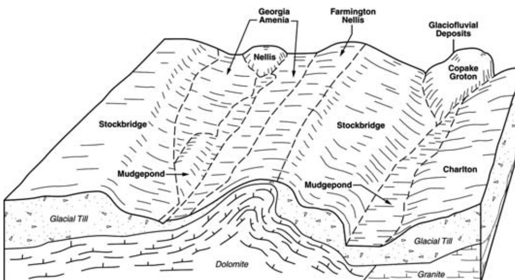
Figure 2.—Typical pattern of soils in the Stockbridge-Charlton-Mudgepond general soil map unit.
