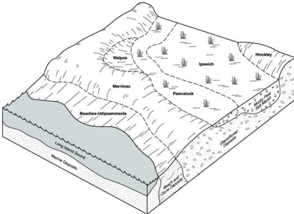
Figure 14.—Typical pattern of soils and parent material in coastal tidal marshes and glaciofluvial areas adjacent to Long Island Sound.
