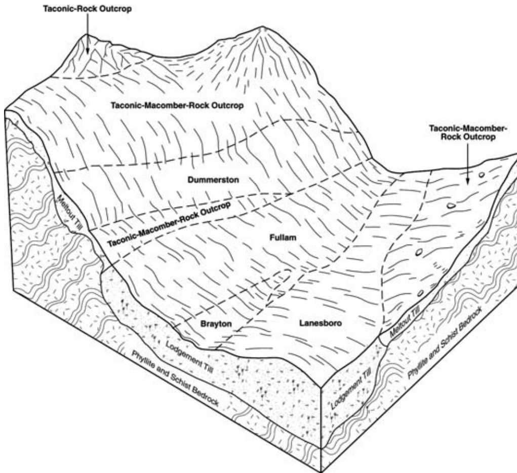
Figure 4.—Typical pattern of soils in the Macomber-Taconic-Lanesboro general soil map unit.
